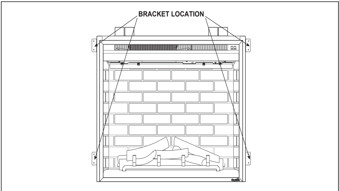
Figure 4.3 Bracket Locations
